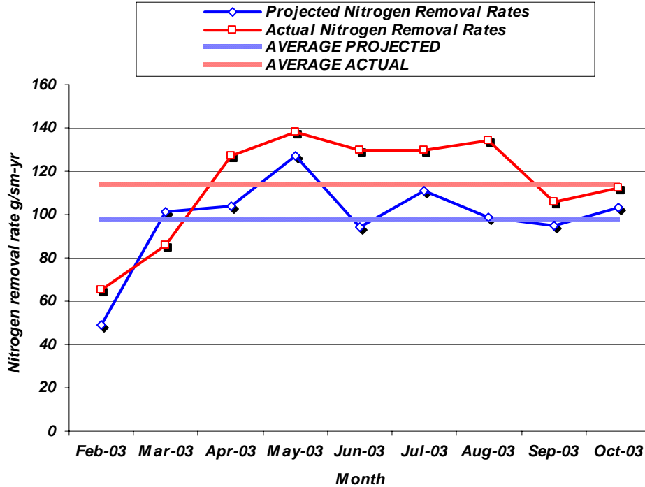
Figure 5-16: S-154 WHST TM actual total nitrogen areal removal rates versus HYDEM model projections for areal removal rates by month through the Q3 monitoring period
