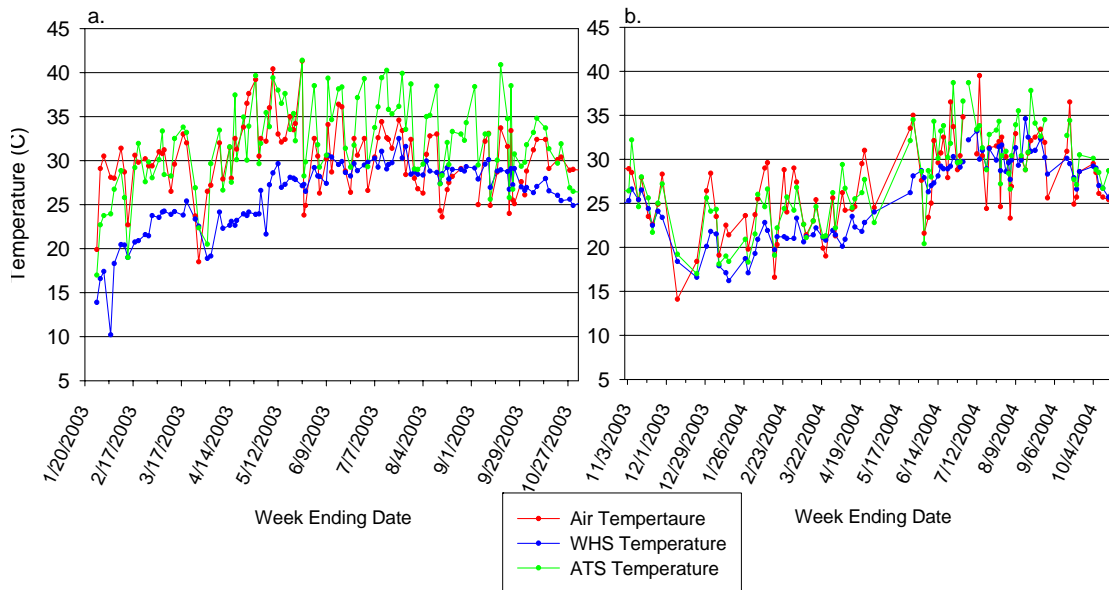
Figure 2-7: Comparative ambient air and water temperature trends as recorded for the afternoon, representing the period of record from January 27, 2003 through October 18, 2004. Figure (a.) represents Quarters 1-3, concentration reduction optimization; Figure (b.) represents Quarters 4-6, load reduction optimization.
