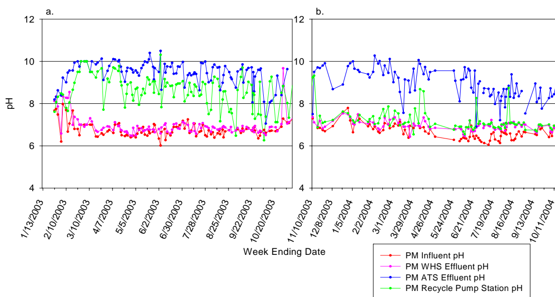
Figure 2-26: PM pH field monitoring stations data for the period of January 27, 2003 through October 18, 2004.
