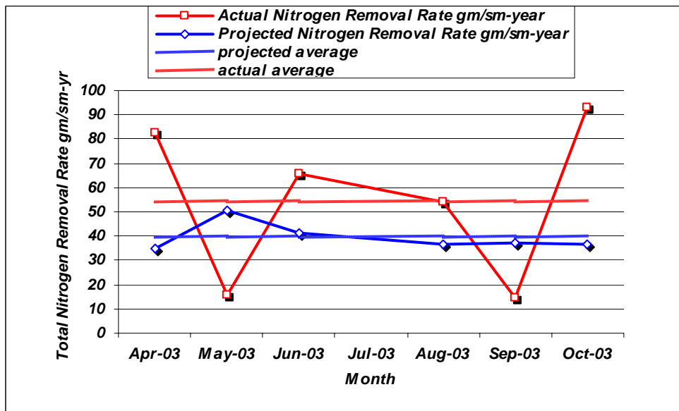
Figure 5-46: ATST TM actual nitrogen areal removal rate versus ATSD-RECYCLE model projections for April through October 2003 monitoring period
