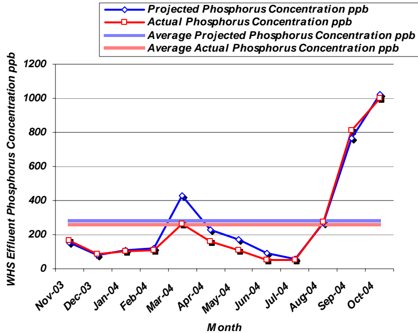
Figure 5-29: S-154 WHSTM actual total phosphorus effluent concentration versus HYDEM model projections for effluent total phosphorus concentration by month for the Q4 through Q6 monitoring period
