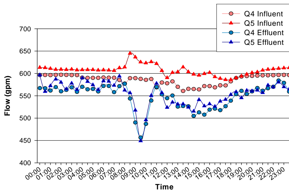
Figure 2-6: Comparative influent and effluent composite diurnal flow patterns for Quarters 4 and 5, representing the period of November 3, 2003 through May 31, 2004.
