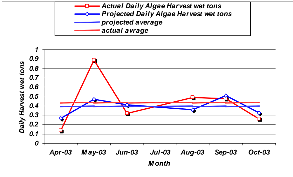
Figure 5-43: ATST ™ actual algae harvest versus ATSDem-RECYCLE model projections for April through October 2003 monitoring period
