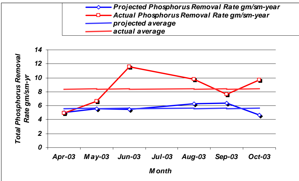
Figure 5-44: ATST ™ actual phosphorus areal removal rate versus ATSDem-RECYCLE model projections for April through October 2003 monitoring period
