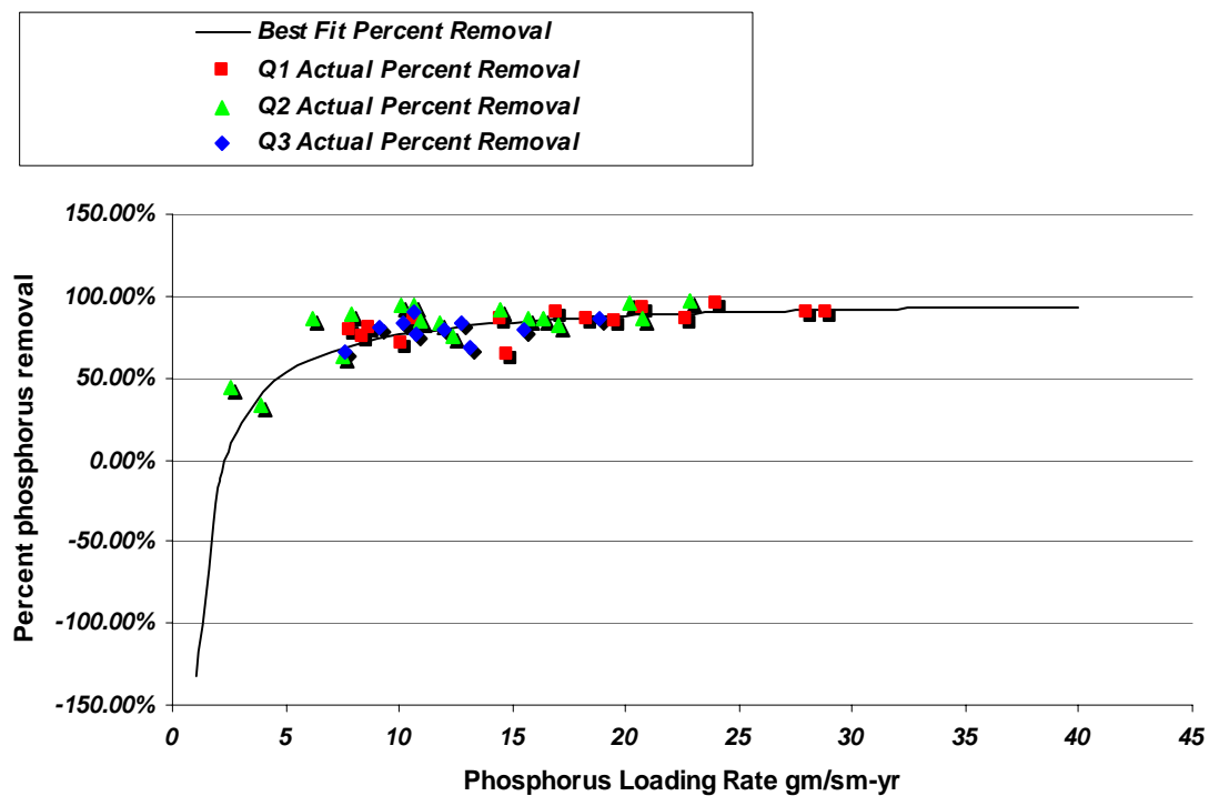
Figure 5-8: S-154 ATST ™ -WHST ™ phosphorus loading rate versus percent phosphorus removal Q1 through Q3.
