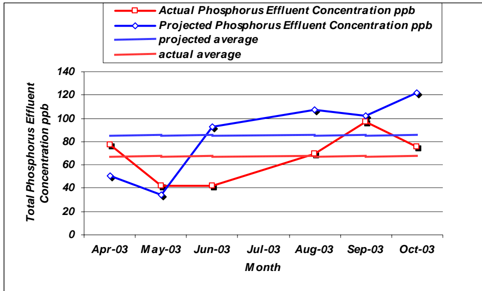
Figure 5-45: ATST TM actual phosphorus effluent concentration versus ATSD-RECYCLE model projections for April through October 2003 monitoring period
