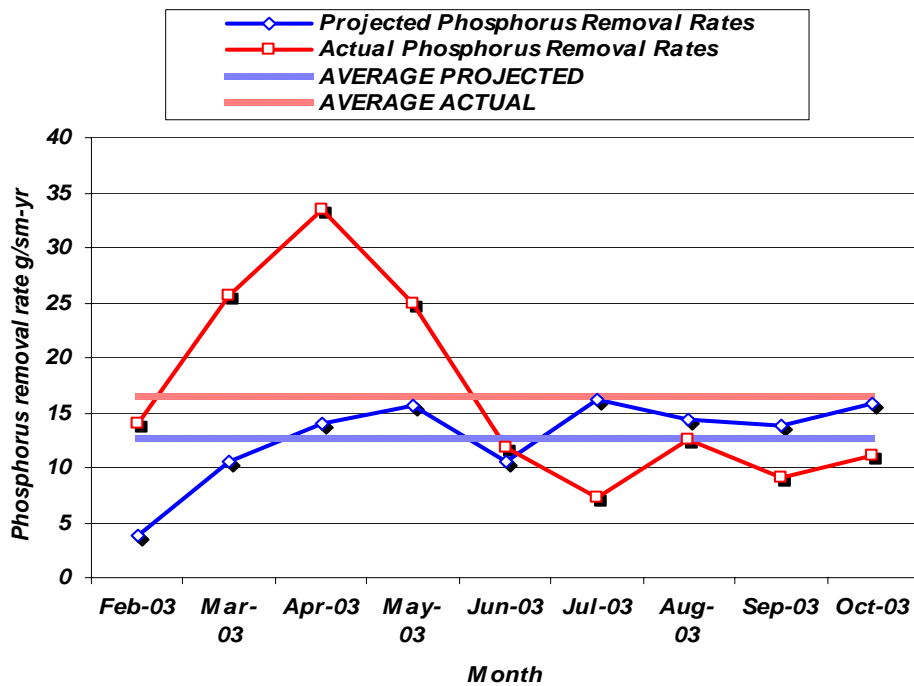
Figure 5-14: S-154 WHST TM actual total phosphorus areal removal rates versus HYDEM model projections for areal removal rates by month through the Q3 monitoring period
